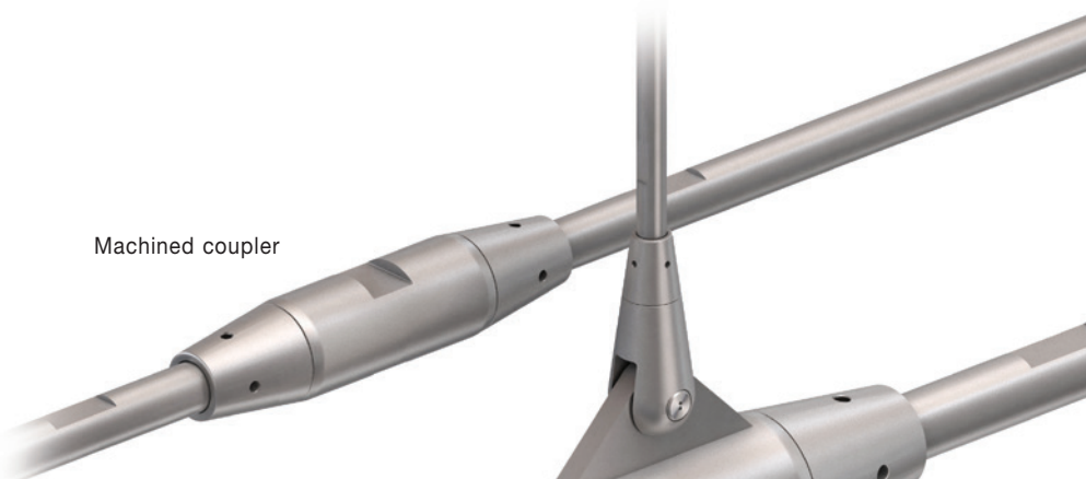
Coupler with hanger to limit the deflection of long tension bars
